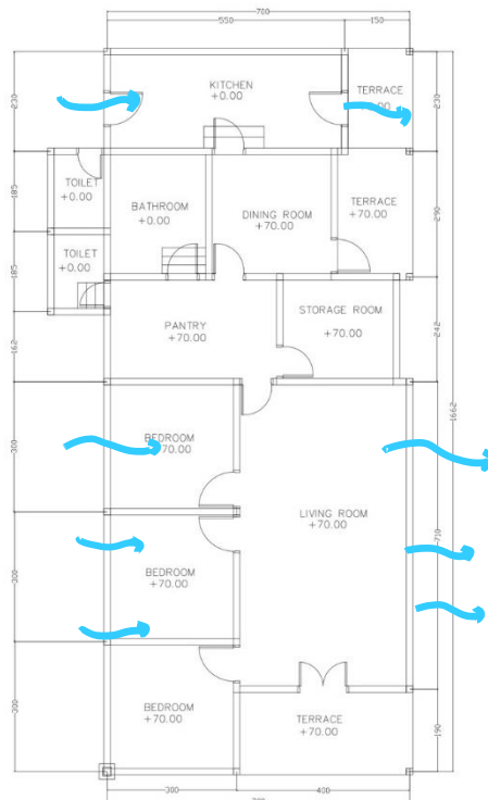
Figure 6. Floor plan of Traditional House and the breeze flow (Author Documentation)
